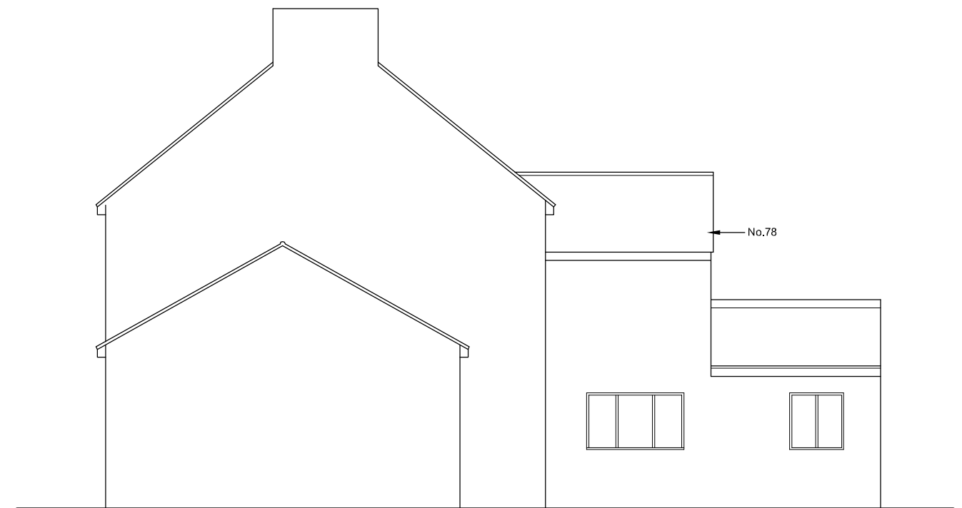
SECTION A-A EXISTING NORTH ELEVATION 1:100
